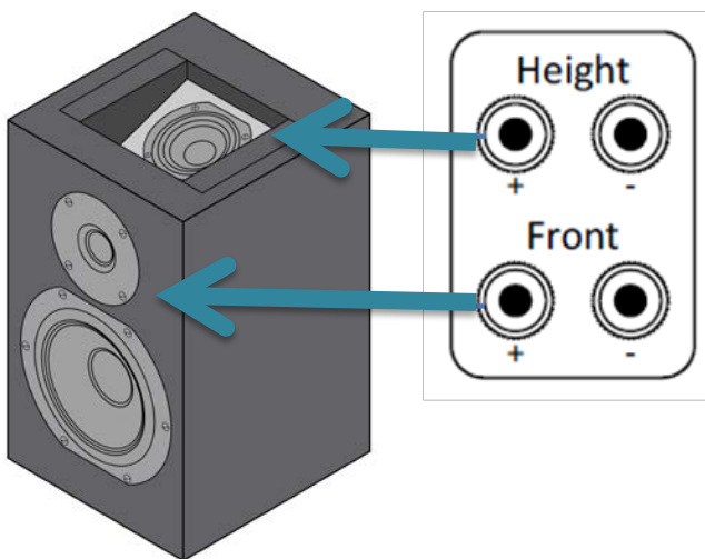
Figure 3: Integrated Dolby Atmos enabled speakers include both traditional drivers and upward-firing elements in the same cabinet. The two sets of speakers have individual posts.
