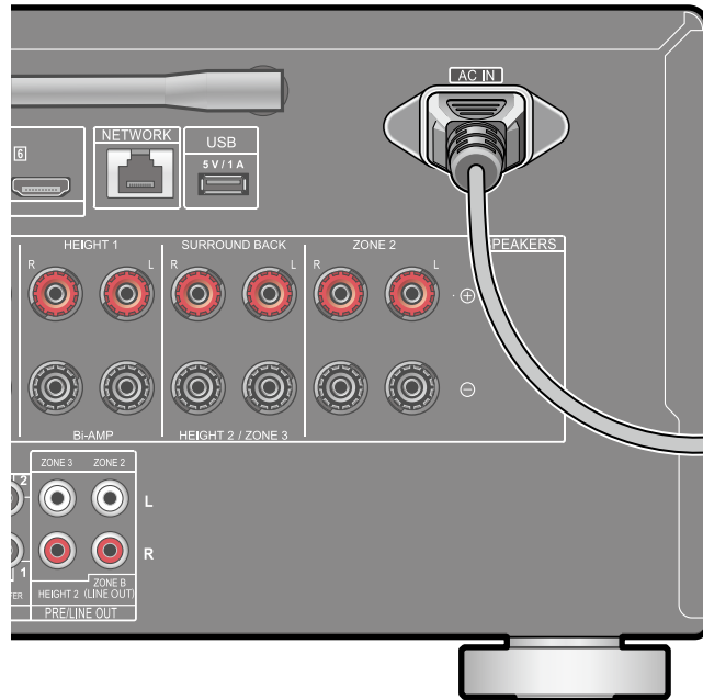
a Power cord
