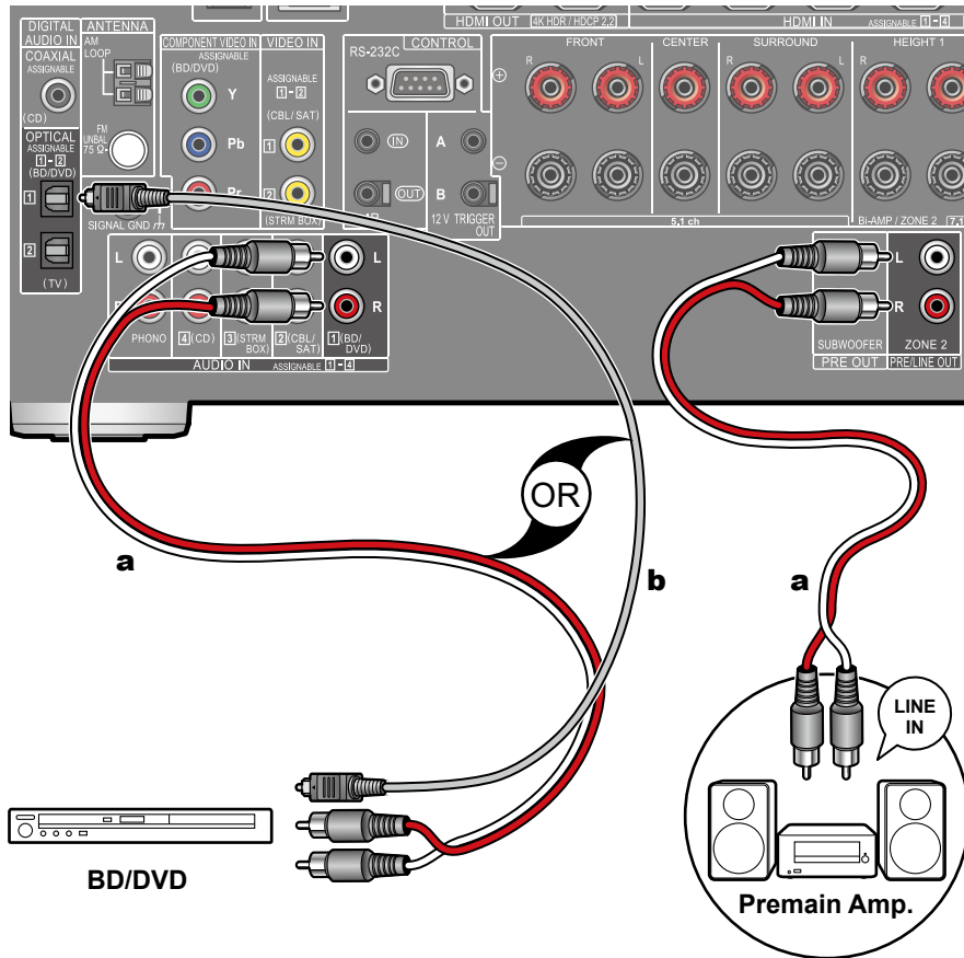
a Analog audio cable, b Digital optical cable
