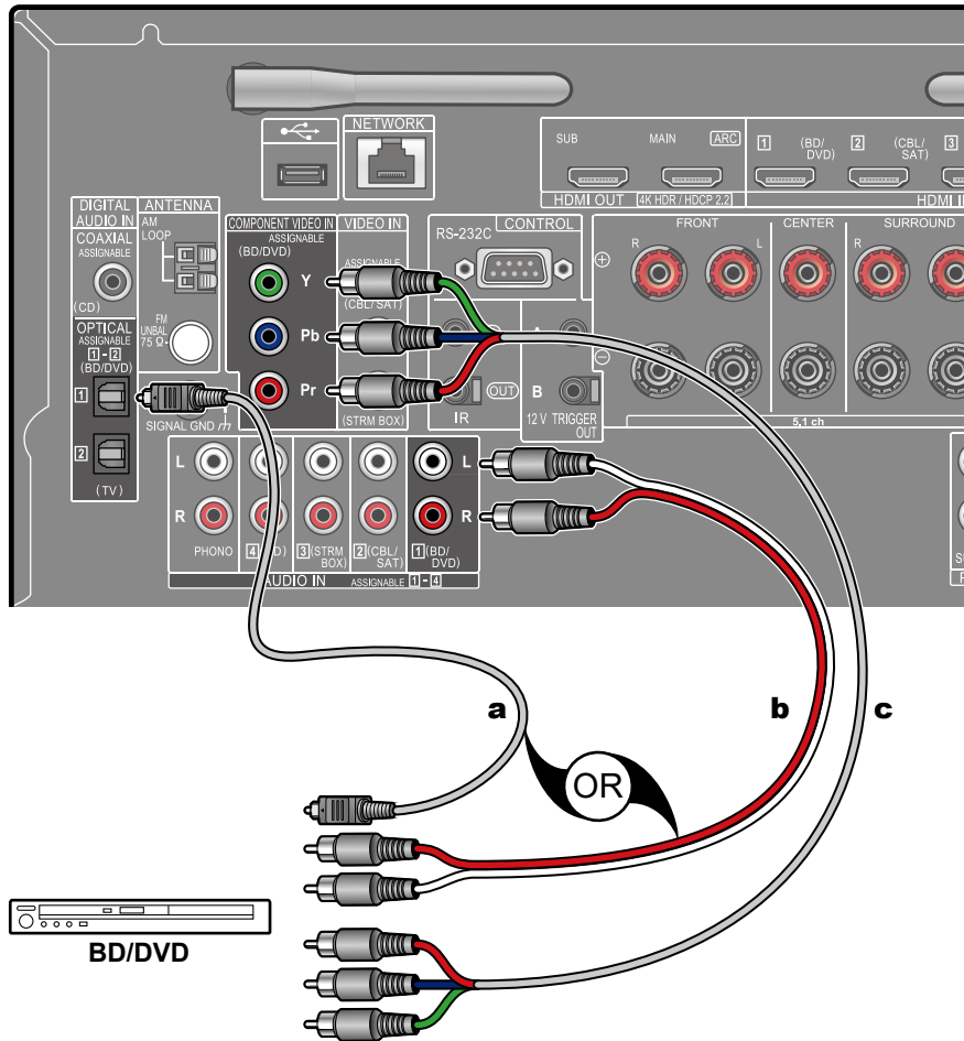
a Digital optical cable, b Analog audio cable, c Component video cable
